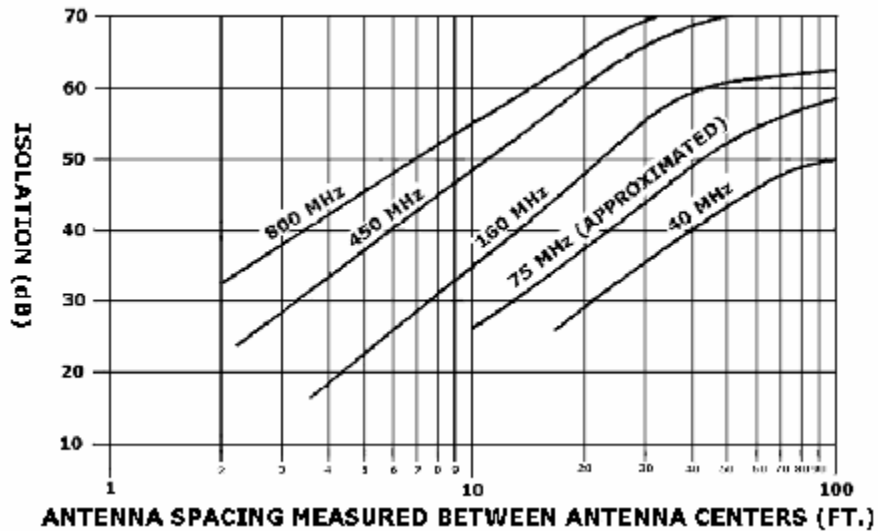
ATTENUATION PROVIDED BY VERTICAL SEPARATION OF DIPOLE ANTENNAS
